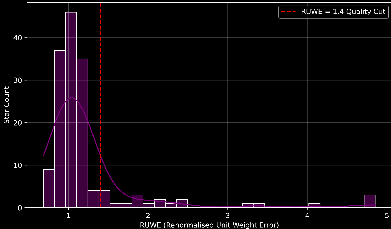
GALAH DR4 Field [7204] RUWE Distribution (n= 152)
