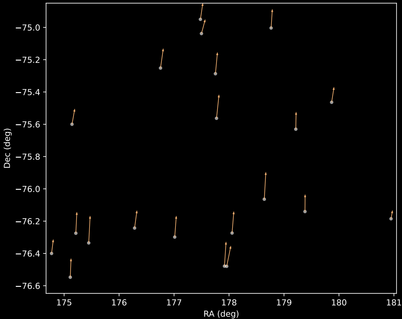
GALAH DR4 Cluster 3 Proper Motion Vectors (n=21)
