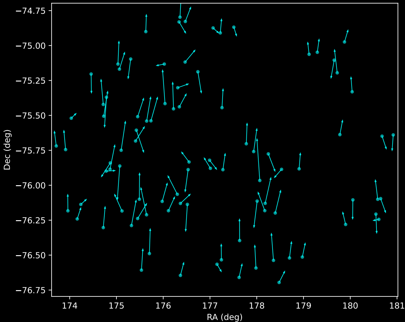
GALAH DR4 Noise Stream Proper Motion Vectors (n=91)
