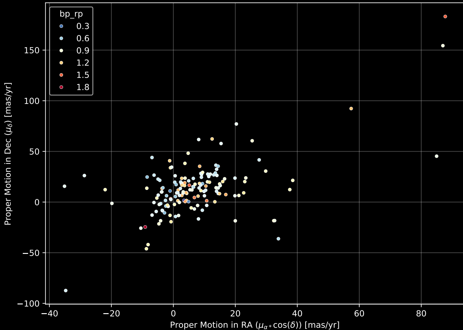
GALAH DR4 Field: [7204] Proper Motion Diagram (n= 158)
