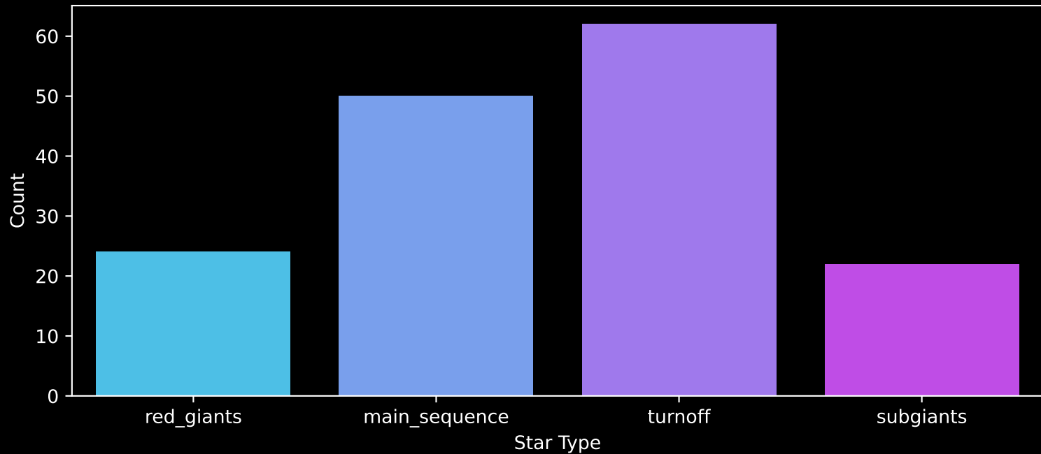
GALAH DR4 Field: [7204] Count plot of Star Type
