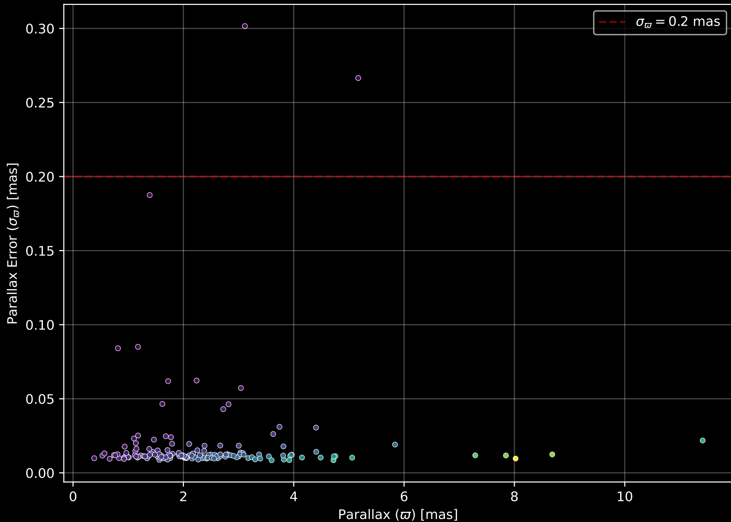
GALAH DR4 Field: [7204] Parallax Quality (n= 158)
